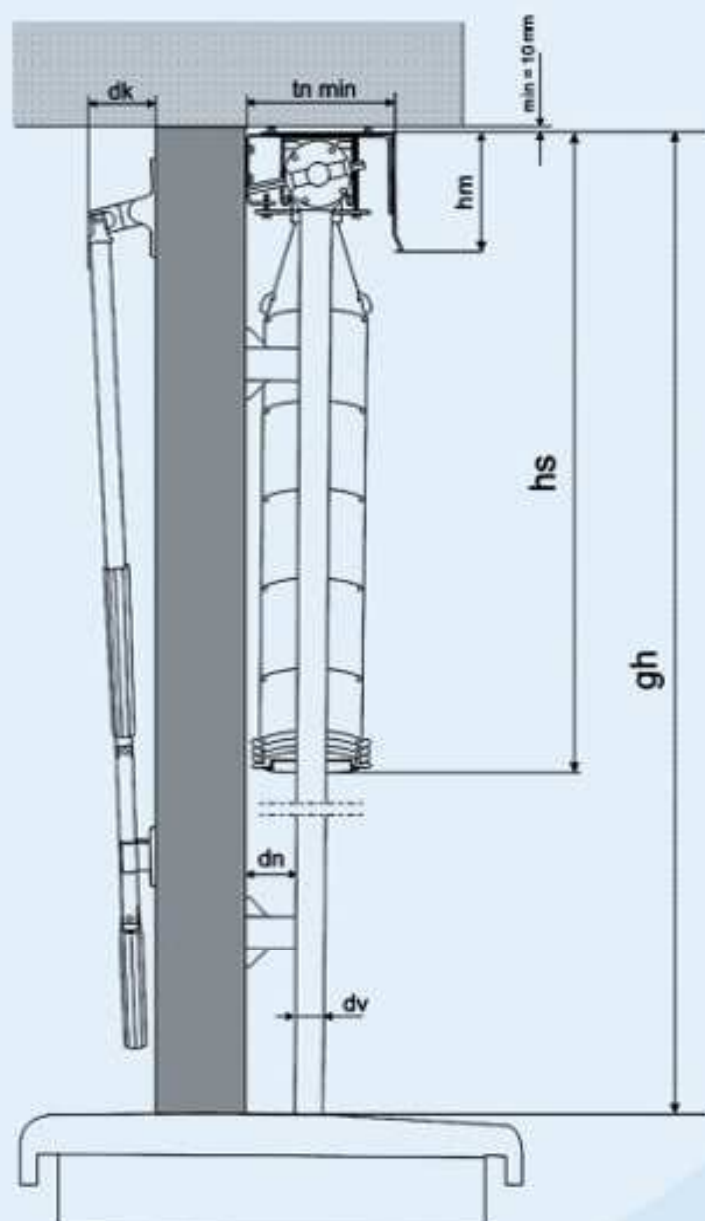
Presek solomatic-a
